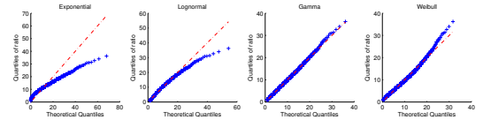
Figure 1: QQ plot of exponential, lognormal, Gamma and Weibull distribution fits for the number of syllables in individual prosodic phrases for Hindi
